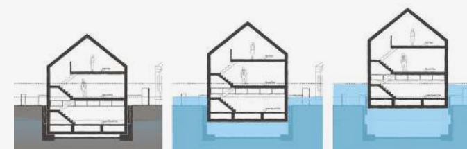
FIGURE 6 Maison amphibie, Buckinghamshire, Royaume-Uni © BACA Architects https://www.baca.uk.com/amphibioushouse.html
